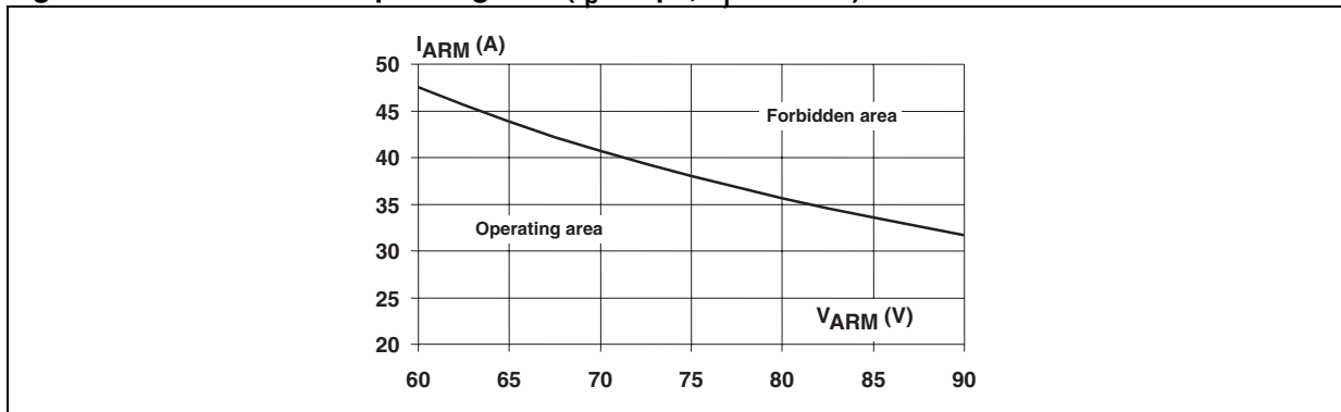
Figure 12. Reverse safe operating area ( t_p < 1 \mu s, T_i > 150 \text{ }^\circ\text{C} )
