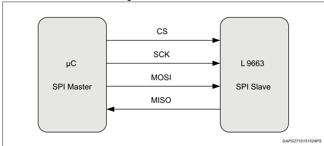
Figure 26. SPI interface
