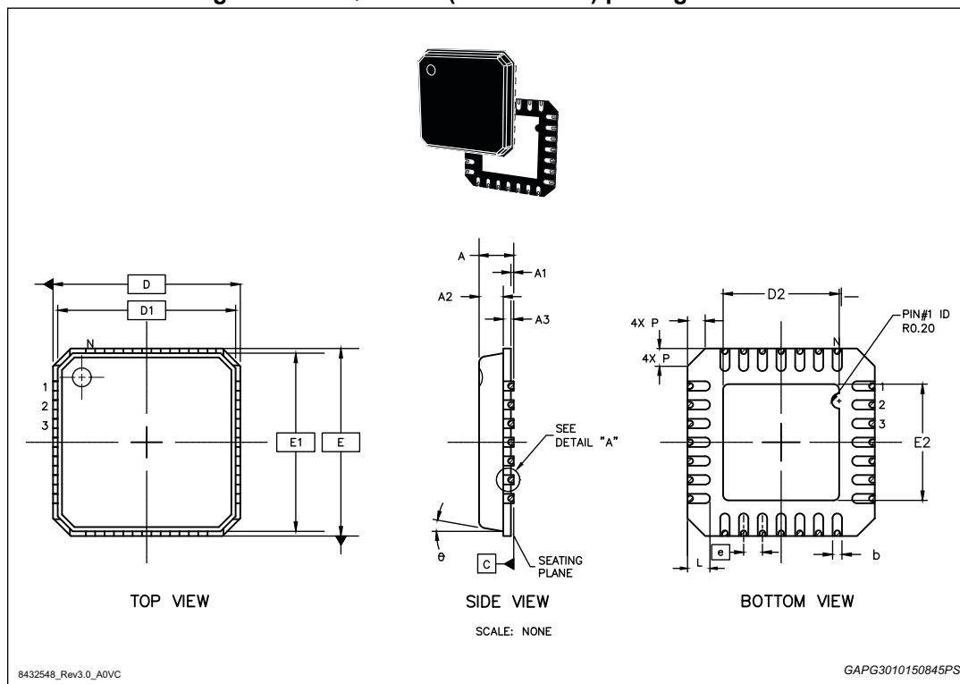
Figure 33. VFQFPN-28 (5x5x1.0 mm) package outline
