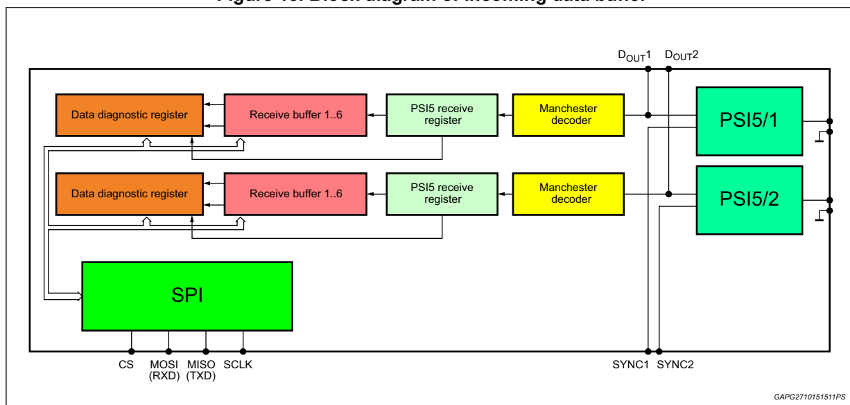
Figure 13. Block diagram of incoming data buffer
