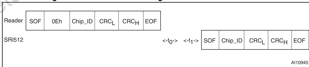
Figure 34. Select frame exchange between reader and SRI512
