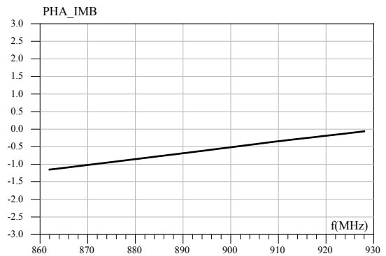
Figure 4. Phase imbalance (°)
