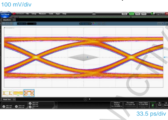
Figure 10: USB3.1 Gen1 5Gbps eye diagram without HSP053-4M5 (with Type-C connector, reference cable and EQ)
