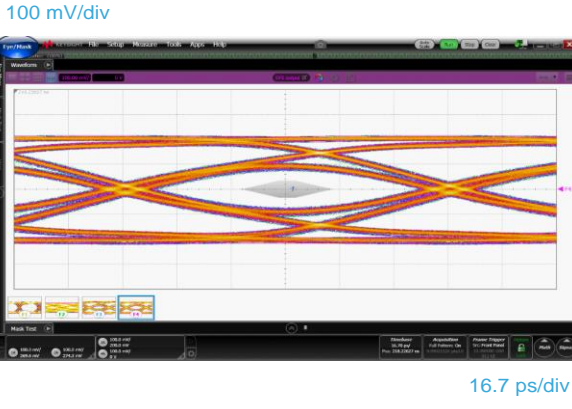
Figure 8: USB3.1 Gen2 10 Gbps eye diagram without HSP053-4M5 (with type-C connector, reference cable, EQ with ADC = 6 dB and DFE)
