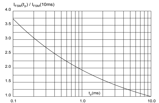
Figure 6. Relative variation of non-repetitive peak surge forward current versus pulse duration (sinusoidal waveform)
