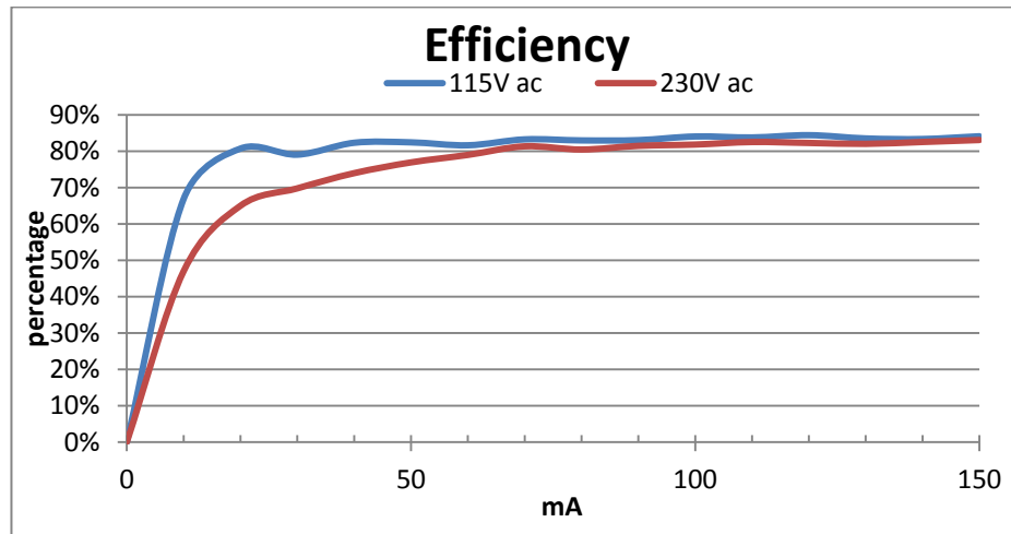
Figure 3. Efficiency measurements
