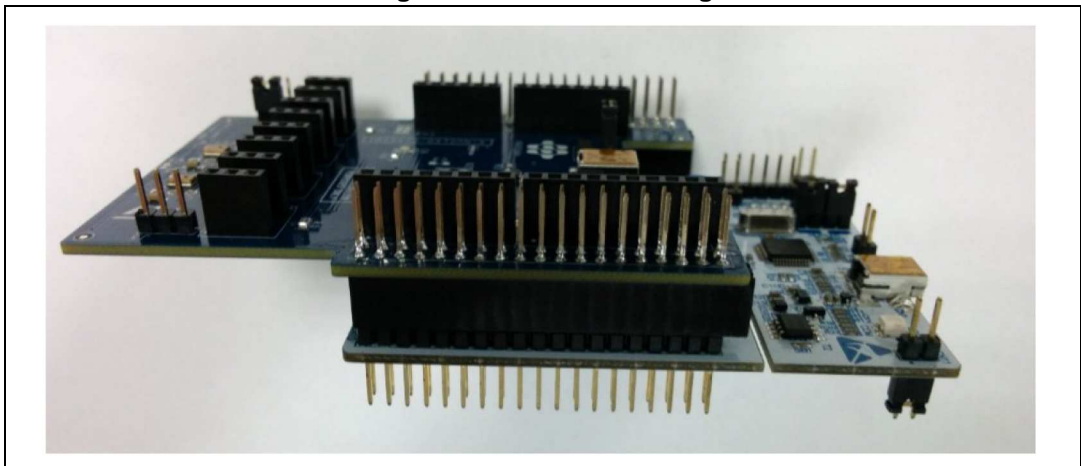
Figure 2. Correct mounting
