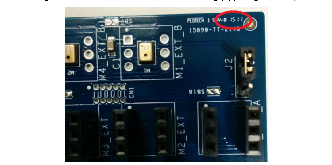
Figure 1. X-NUCLEO-CCA02M1, board marking (upper right corner)
