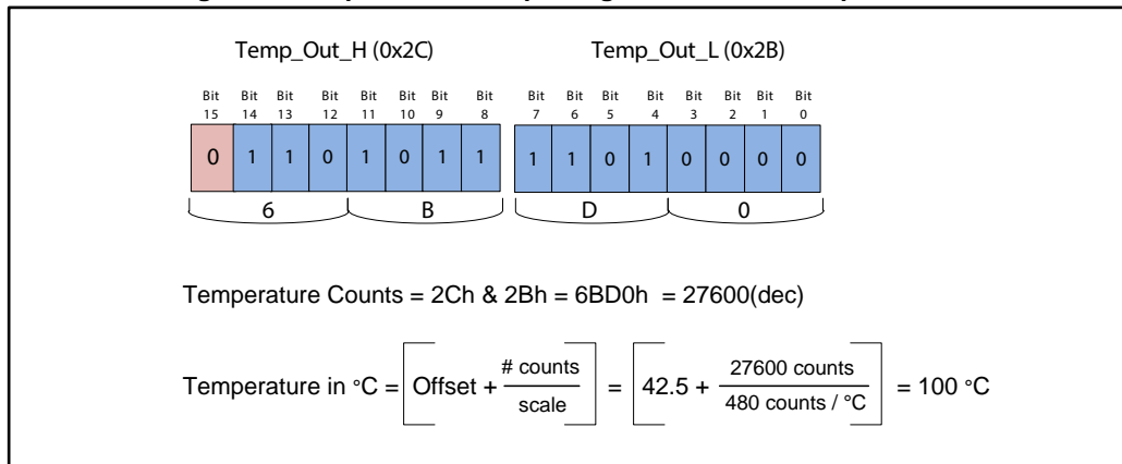
Figure 4: Temperature example: sign bit is 0, this is a positive value
