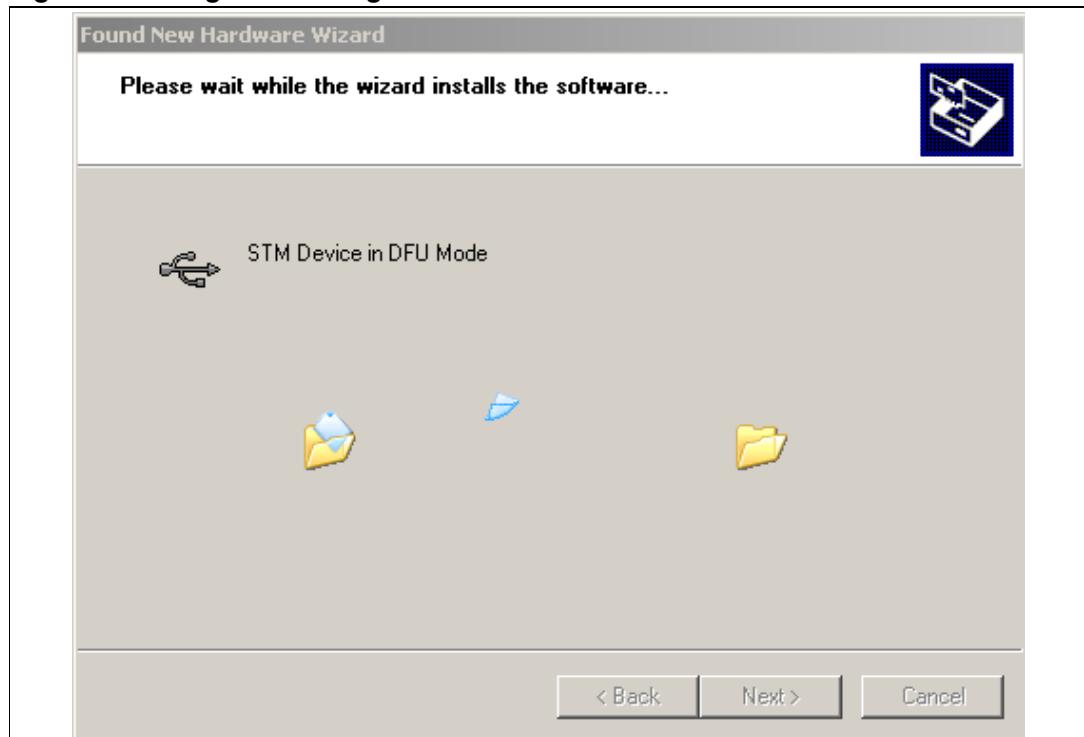
Figure 6. Progress message
