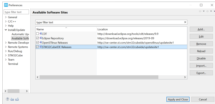
Figure 18. Preferences window
