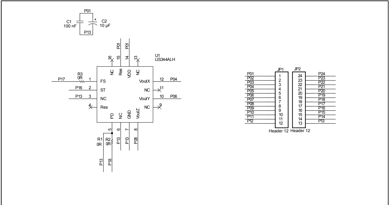
Figure 1: STEVAL-MKI015V1 circuit schematic
