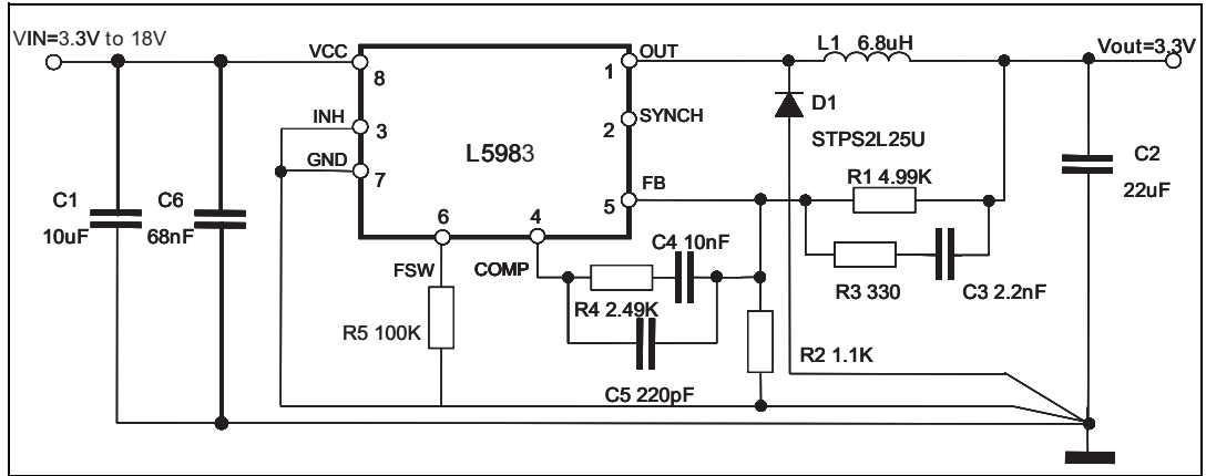
Figure 1. STEVAL-ISA144V1 schematic circuit
