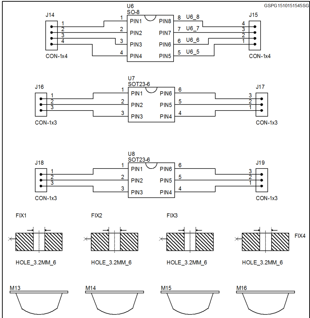
Figure 5: STEVAL-ILL075V1 circuit schematic (5 of 5)
