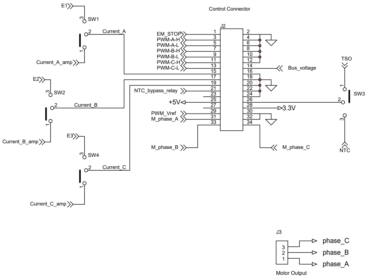
Figure 2: STEVAL-IPM10F circuit schematic (2 of 6)
