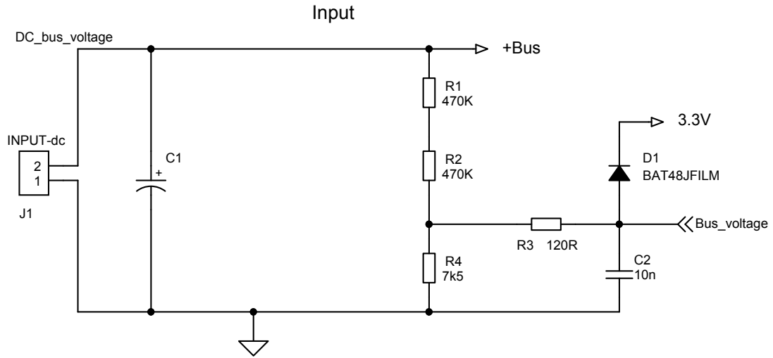
Figure 3: STEVAL-IPM10F circuit schematic (3 of 6)
