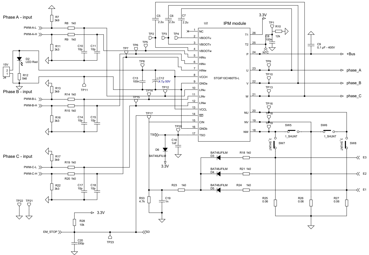
Figure 6: STEVAL-IPM10F circuit schematic (6 of 6)
