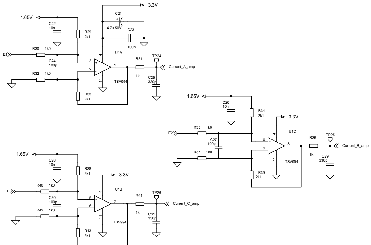
Figure 4: STEVAL-IPM10F circuit schematic (4 of 6)
