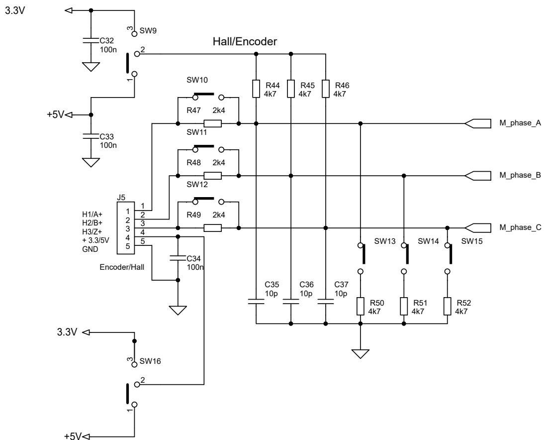
Figure 6: STEVAL-IPM10F circuit schematic (6 of 6)
