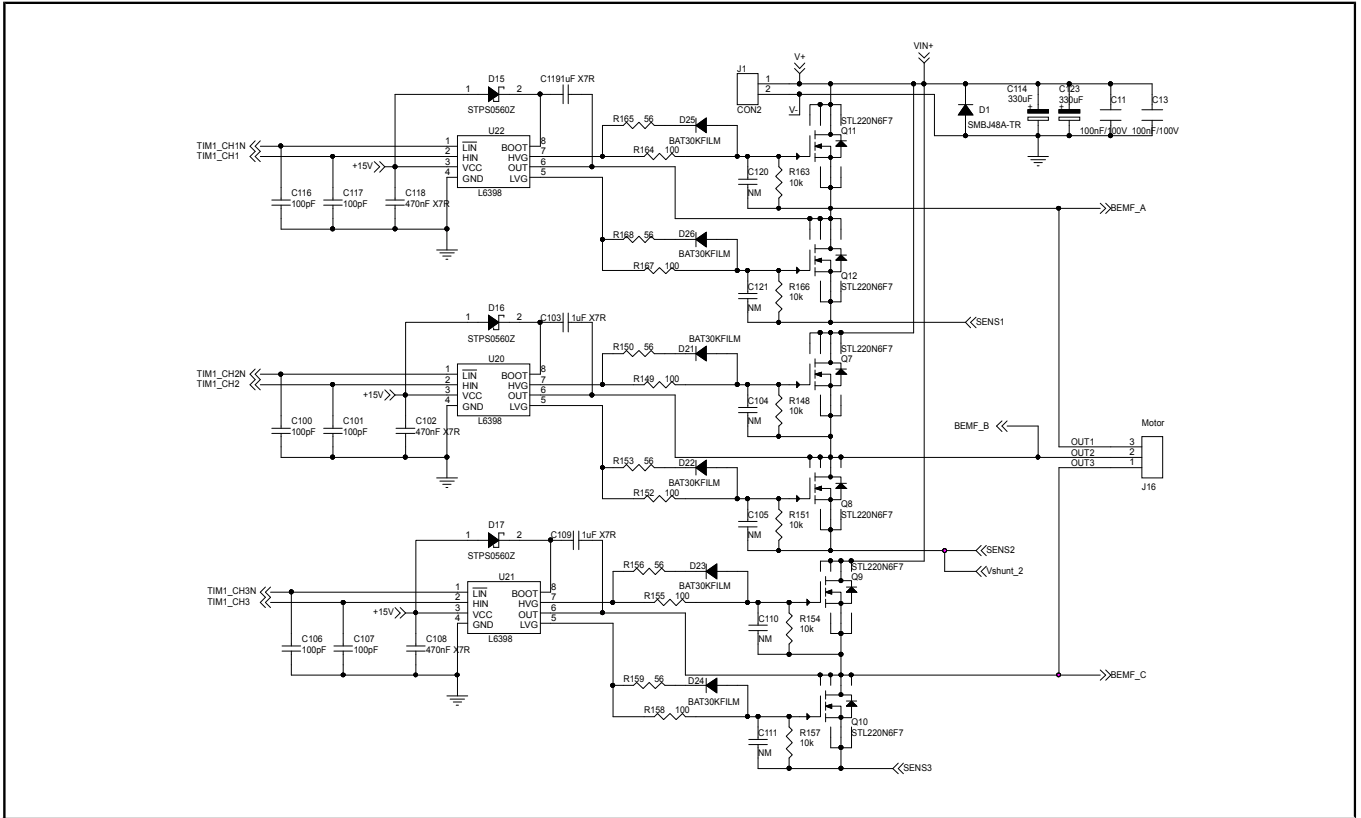
Figure 2: Schematic - Power section (2/2)
