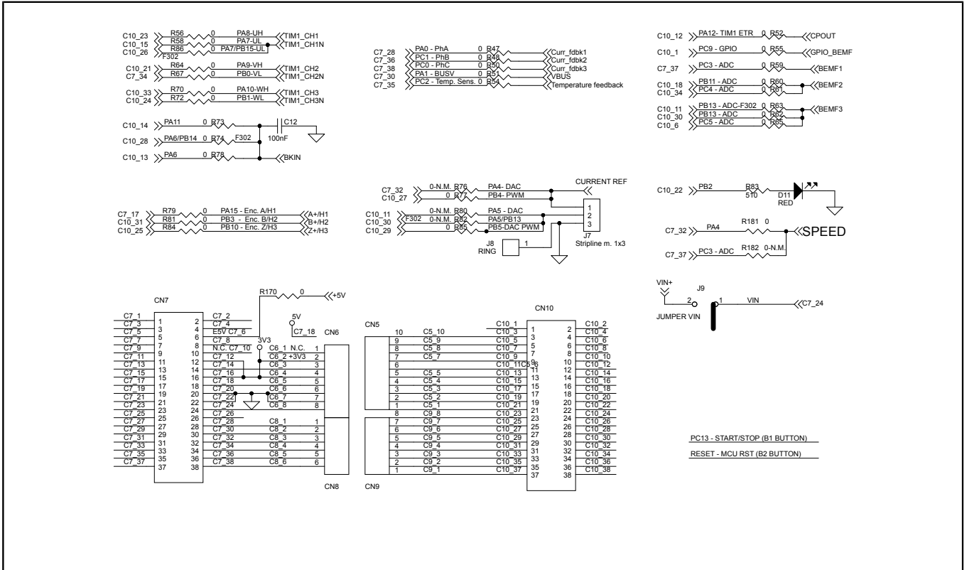
Figure 6: Schematic - MCU pinout assignment
