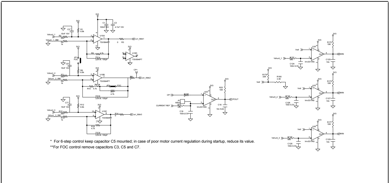
Figure 5: Schematic - Analog conditioning and Current protection circuit
