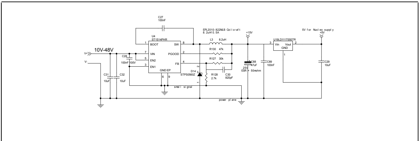
Figure 3: Schematic - Auxiliary power supply circuit
