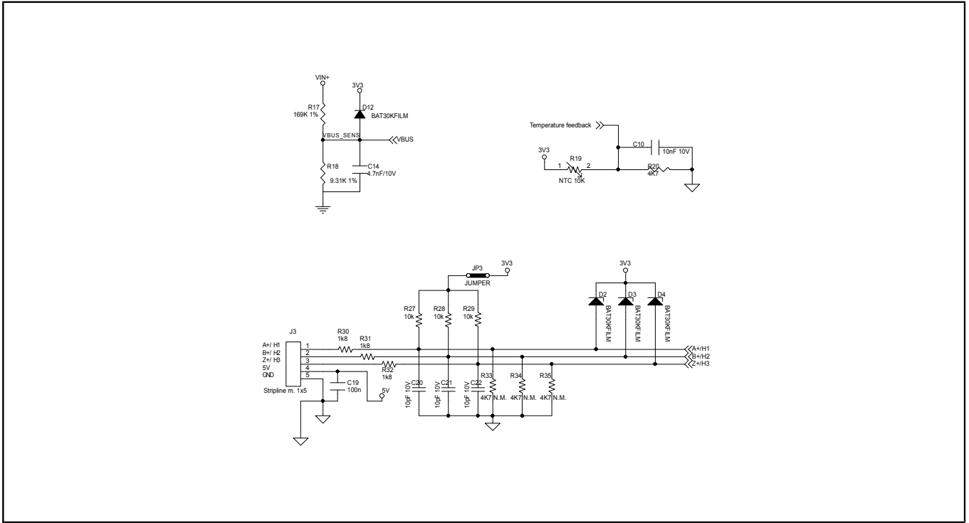
Figure 5: Schematic - Analog conditioning and Current protection circuit
