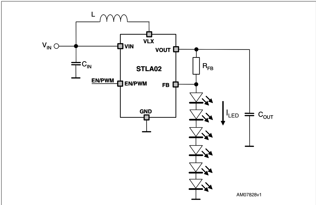
STEVAL-TLL010V1 Schematic diagram
