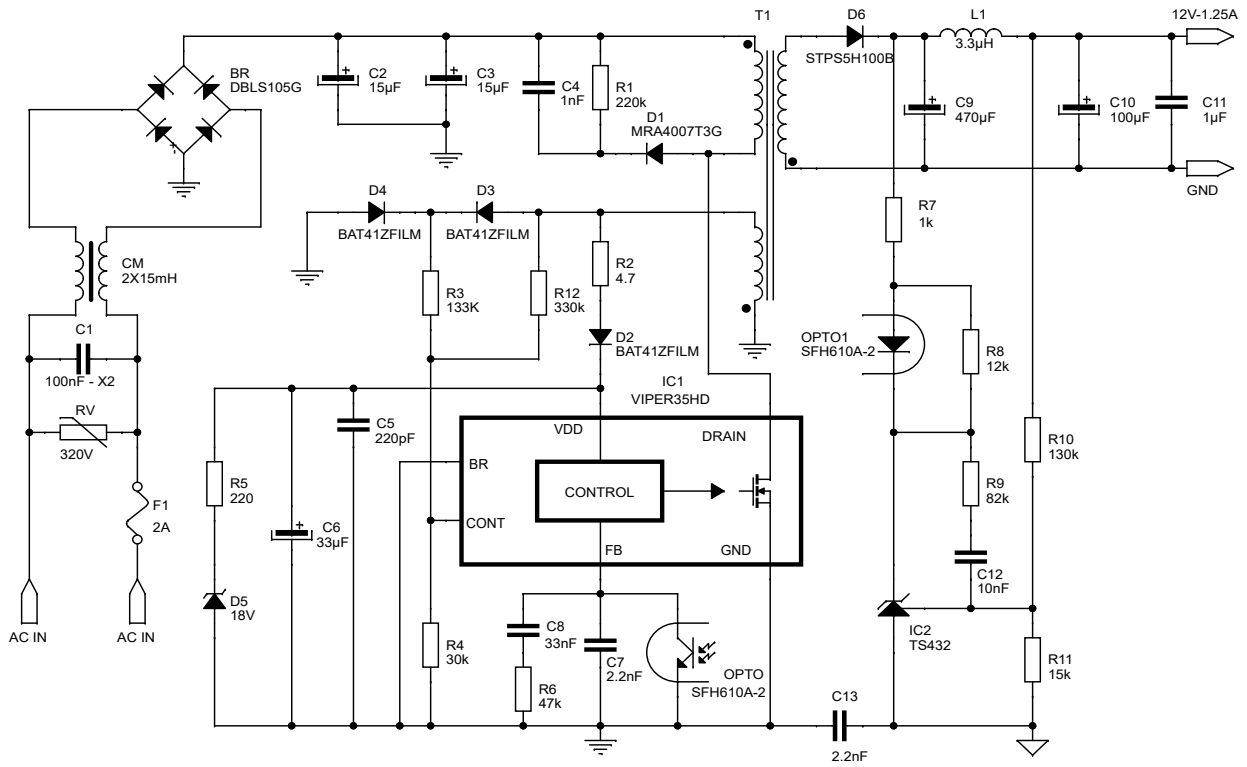
Figure 1: STEVAL-ISA171V1 circuit schematic
