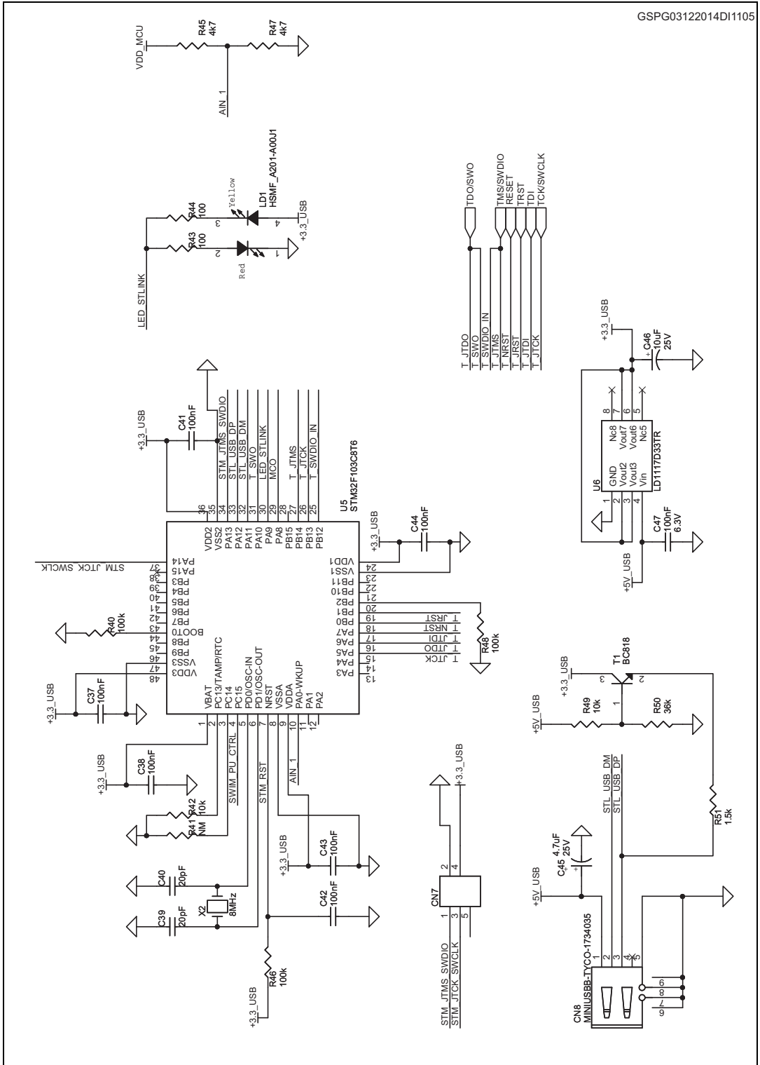
Figure 4. Schematic (4 of 5)
