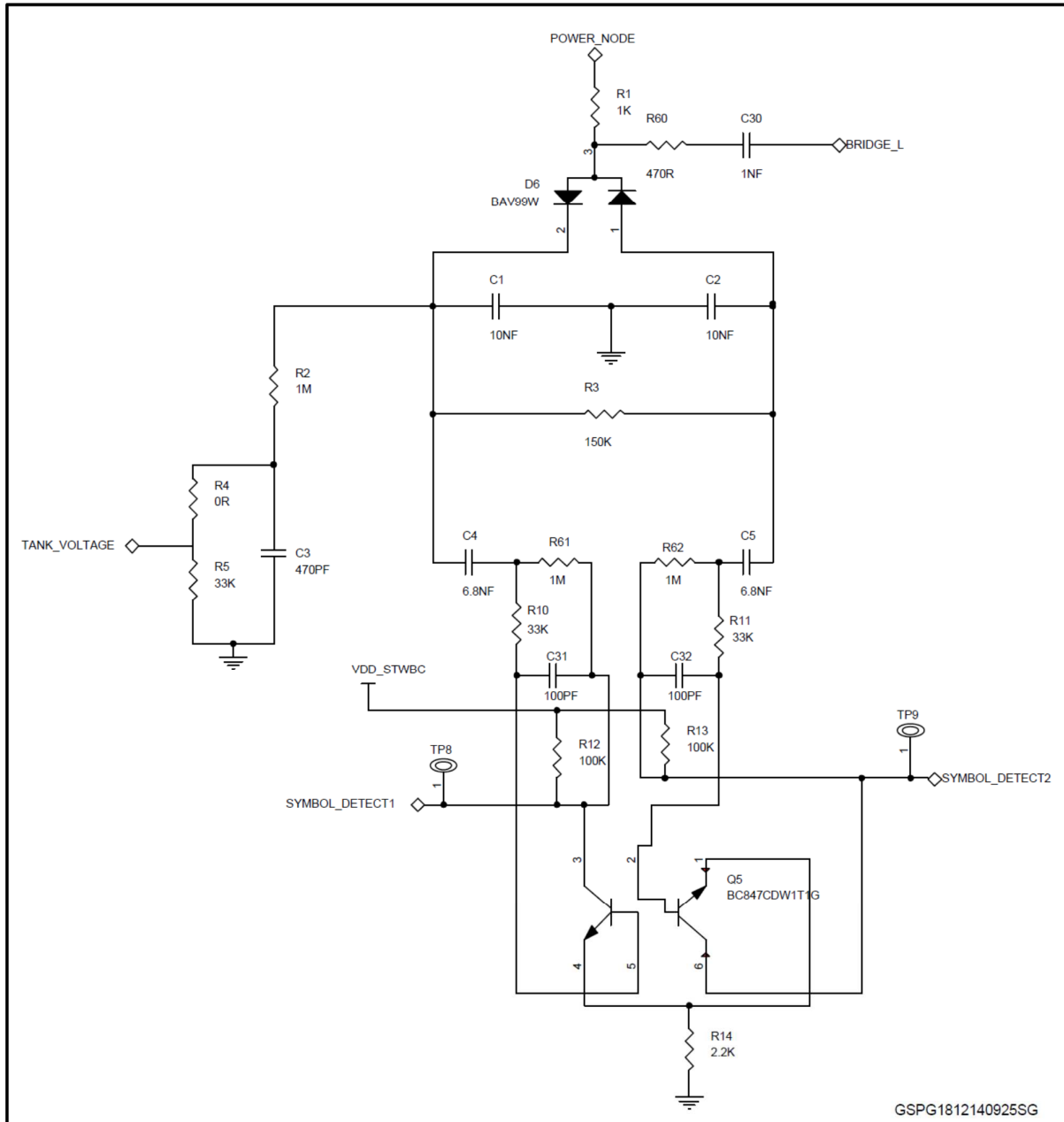
Figure 3: STEVAL-ISB027V1 circuit schematic (3 of 3)
