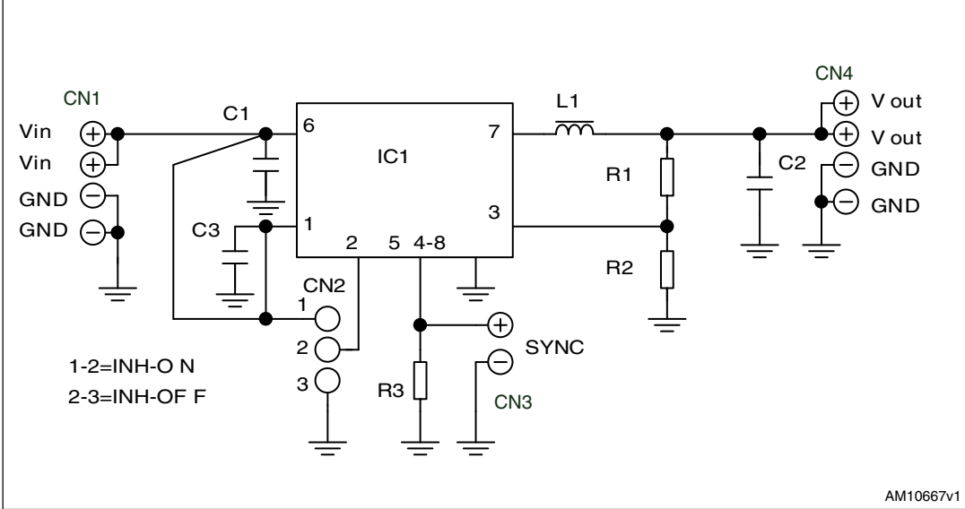
Figure 1. Schematic
