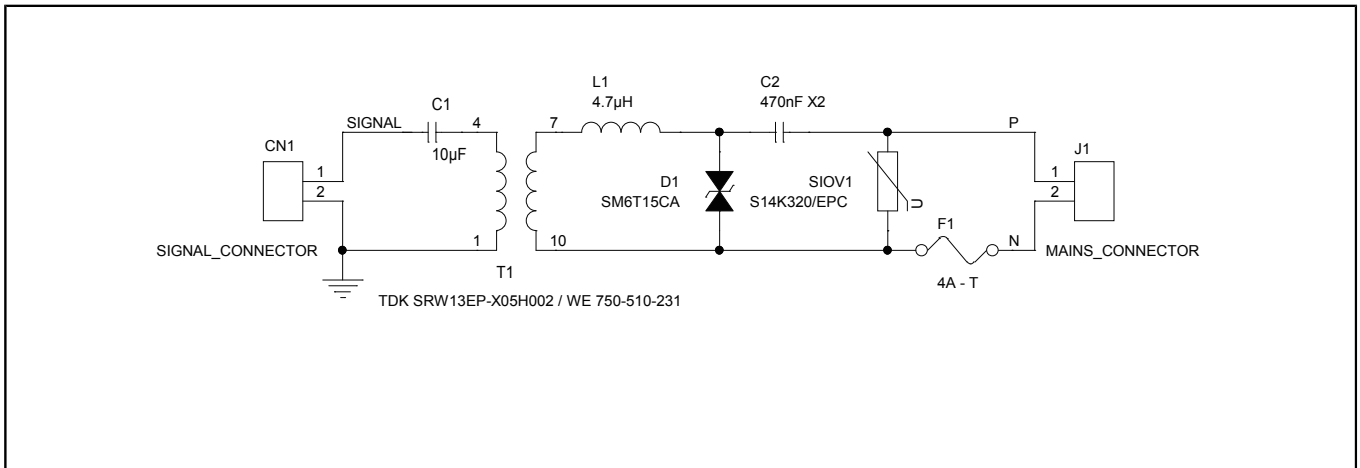
Figure 1: STEVAL-XPLM01CPL circuit schematic
