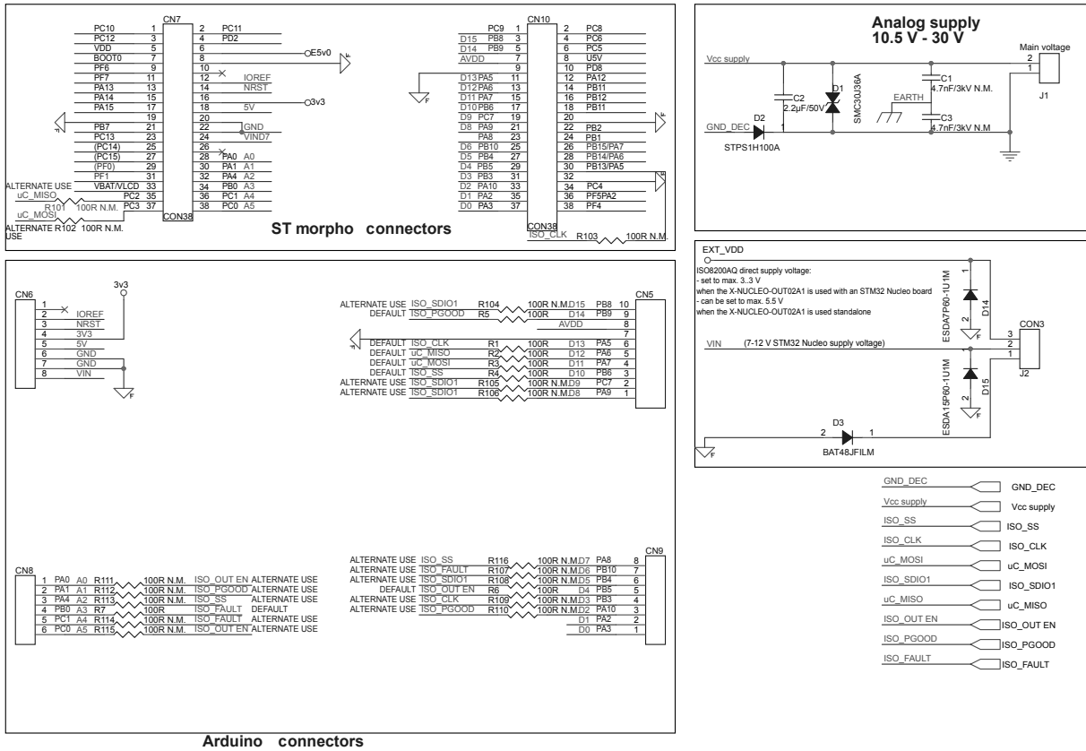
Figure 2: X-NUCLEO-OUT02A1 circuit schematic (2 of 2)
