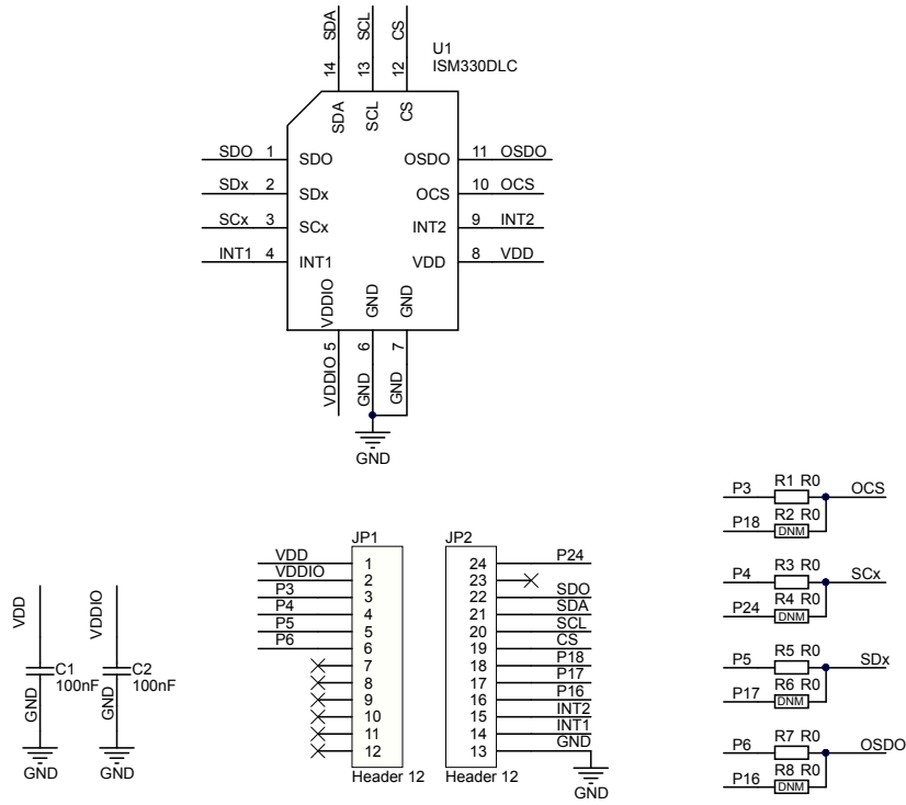
Figure 1: STEVAL-MKI182V2 circuit schematic
