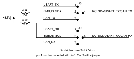
Figure 7: STEVAL-DPSADP01 adapter board schematic
