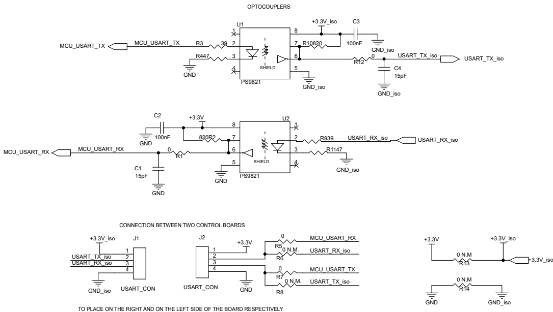
Figure 6: STEVAL-DPS334C1 control board - opto-isolated communication schematic
