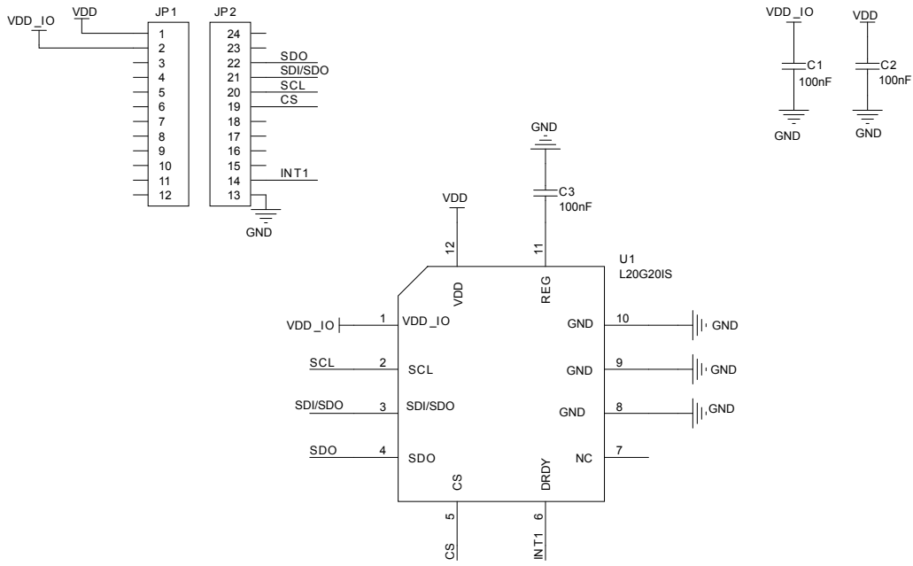
Figure 1: STEVAL-MKI188V1 circuit schematic
