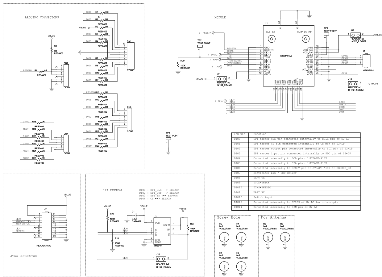
Figure 2: STEVAL-FKI001V1 board schematic (2 of 2)
