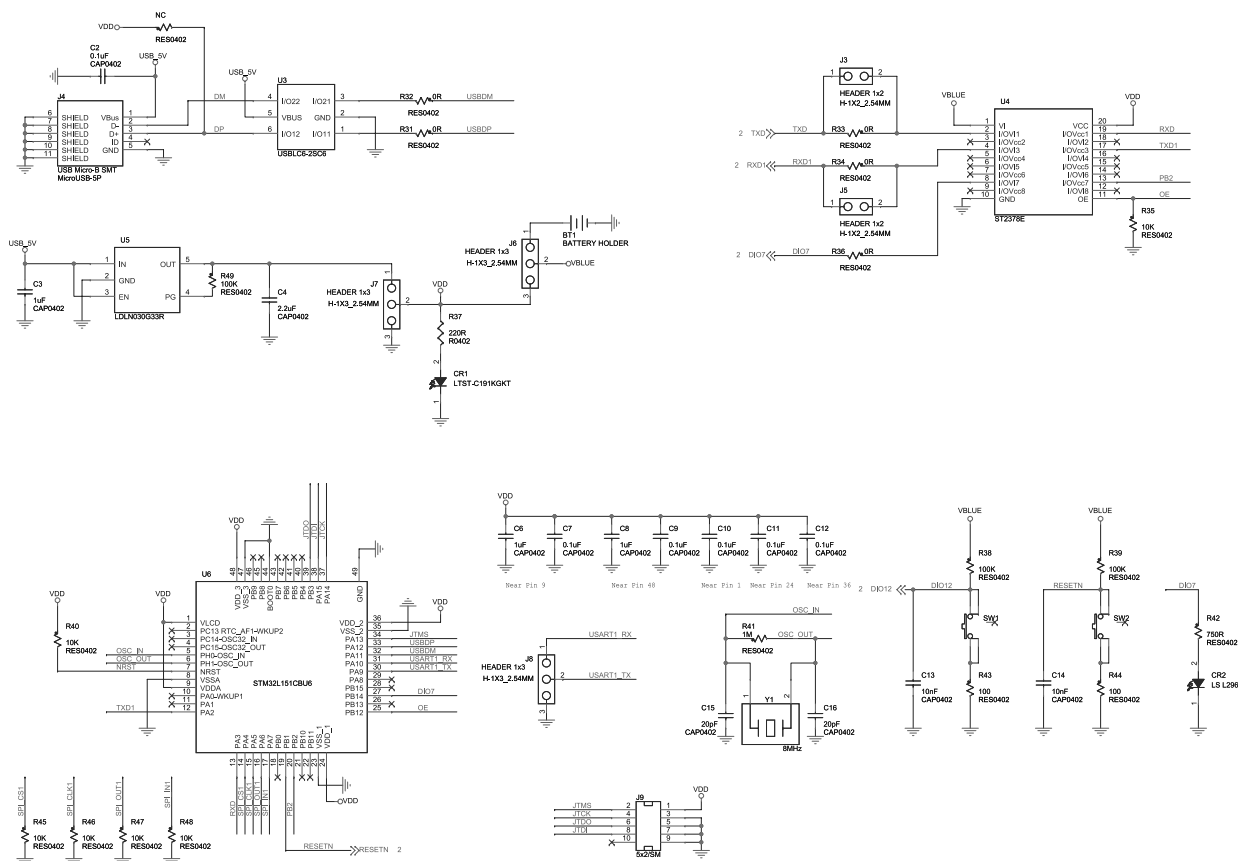
Figure 2: STEVAL-FKI001V1 board schematic (2 of 2)
