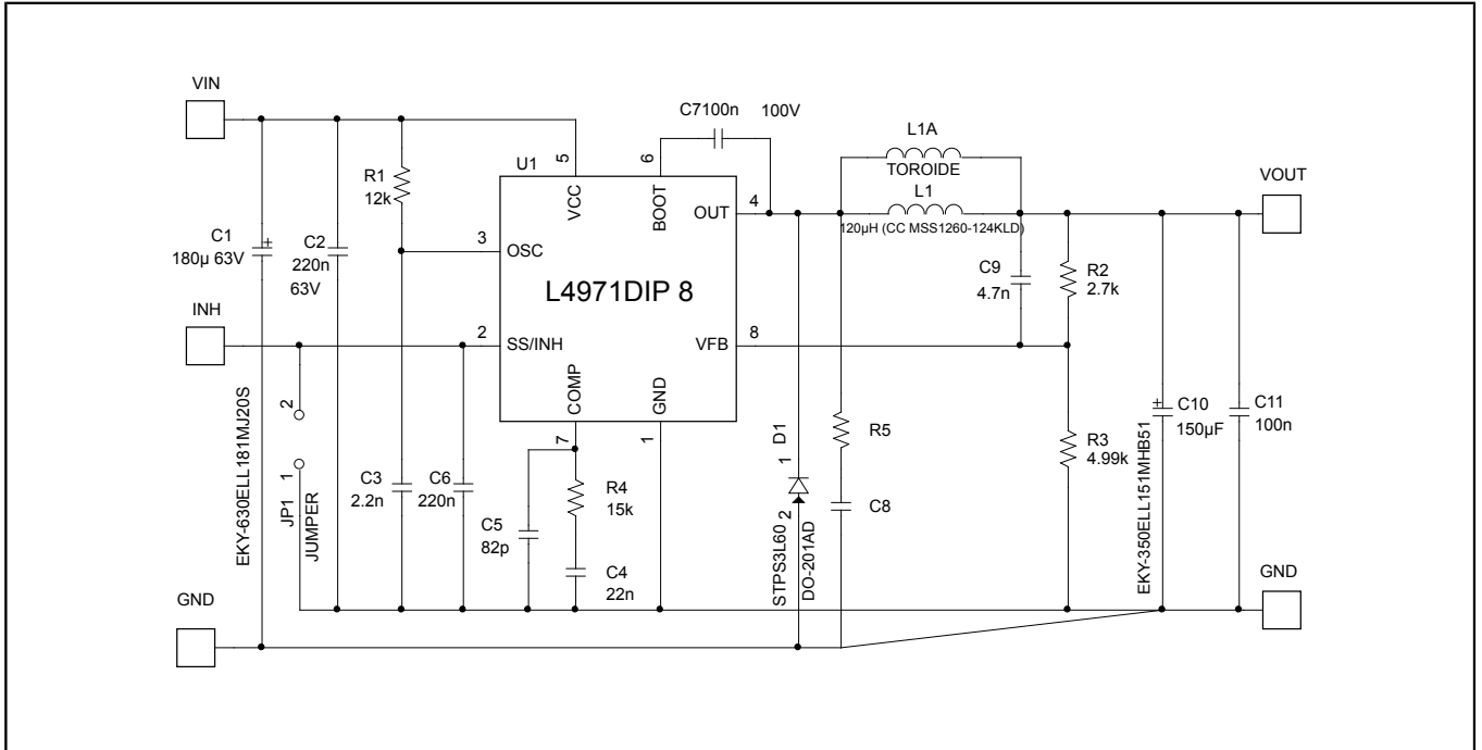
Figure 1: STEVAL-ISA202V1 circuit schematic
