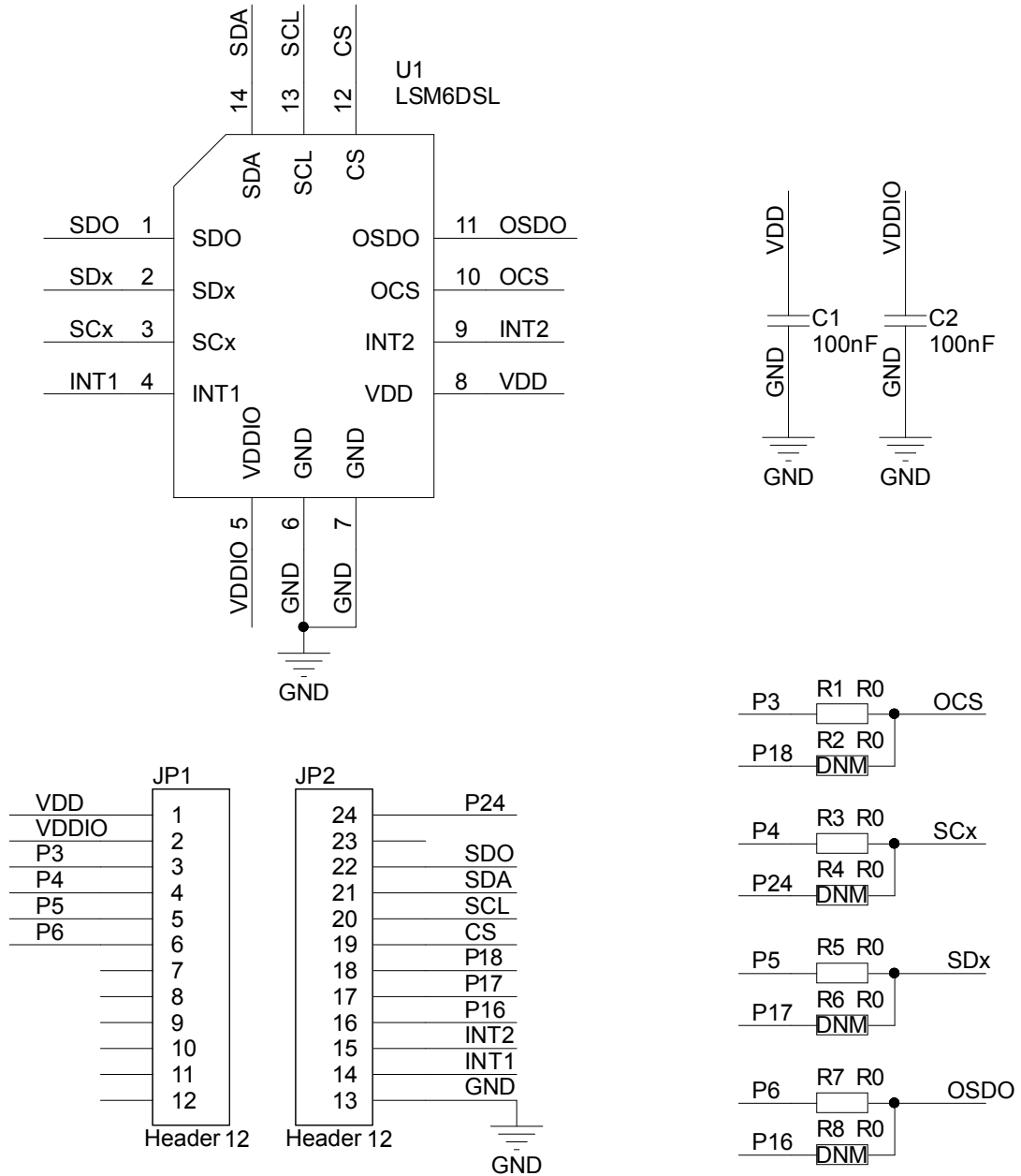
Figure 1: STEVAL-MKI178V2 circuit schematic
