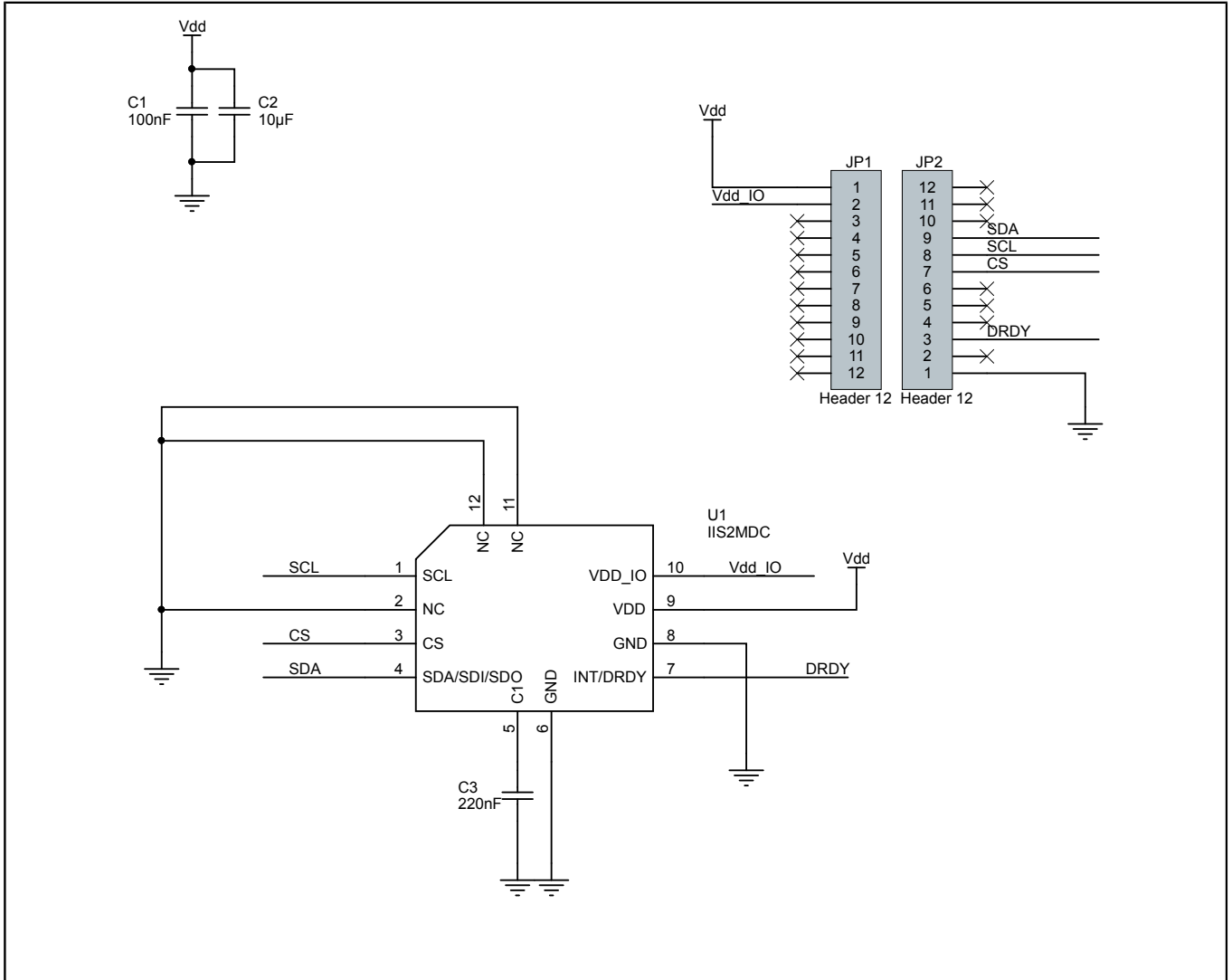
Figure 1: STEVAL-MKI185V1 - circuit schematic
