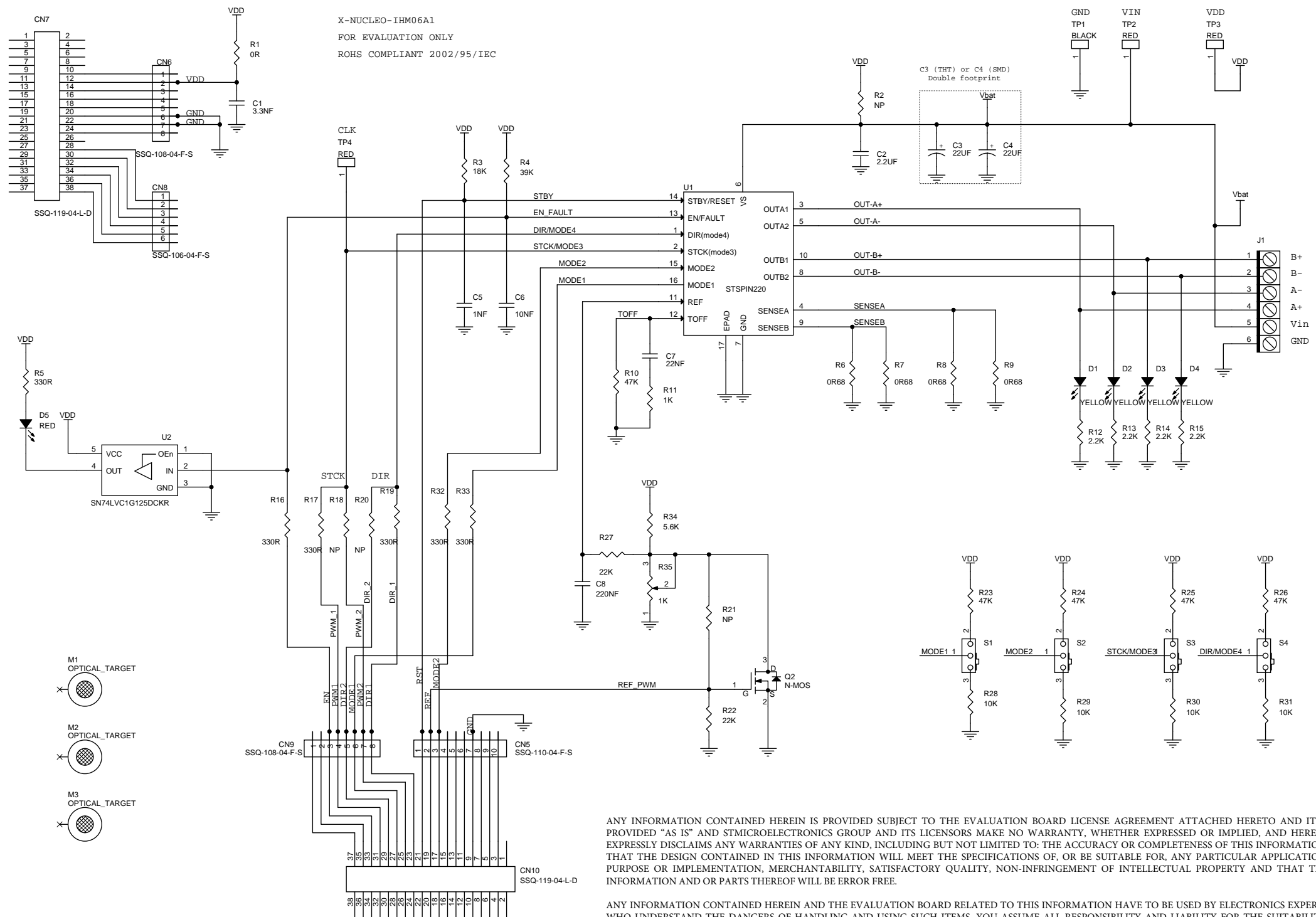
Circuit Schematic (1/1) - X-NUCLEO-IHM06A1
