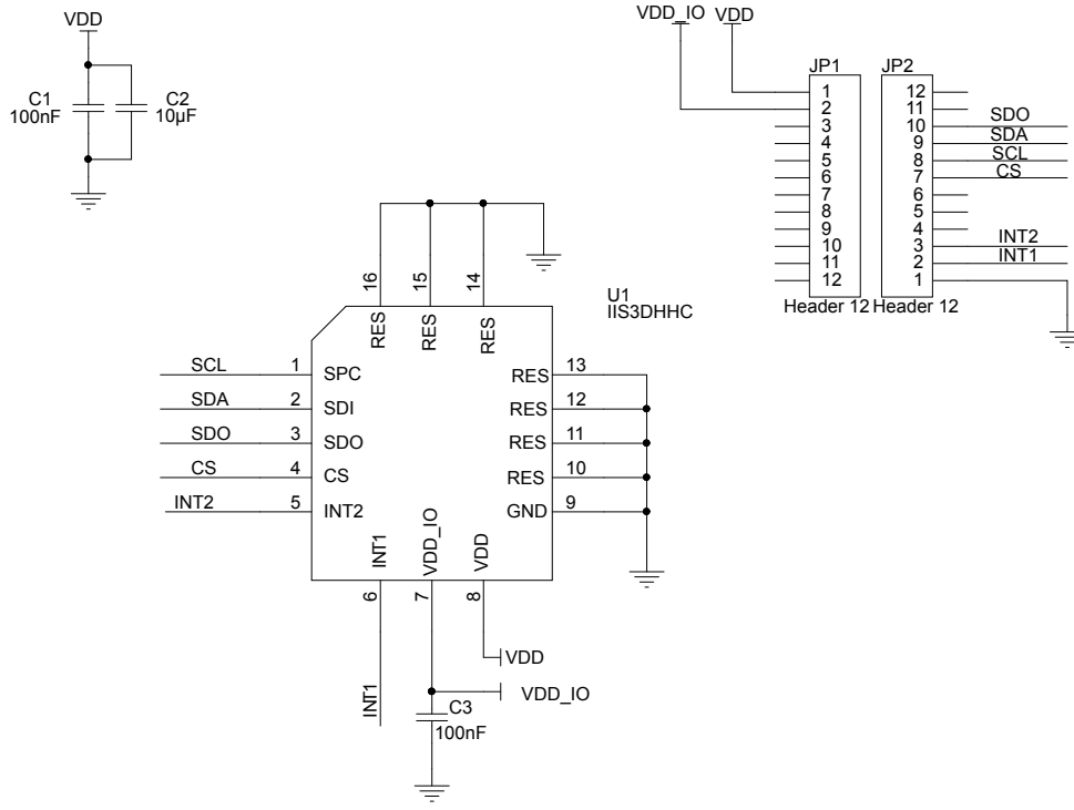
Figure 1: STEVAL-MKI186V1 circuit schematic
