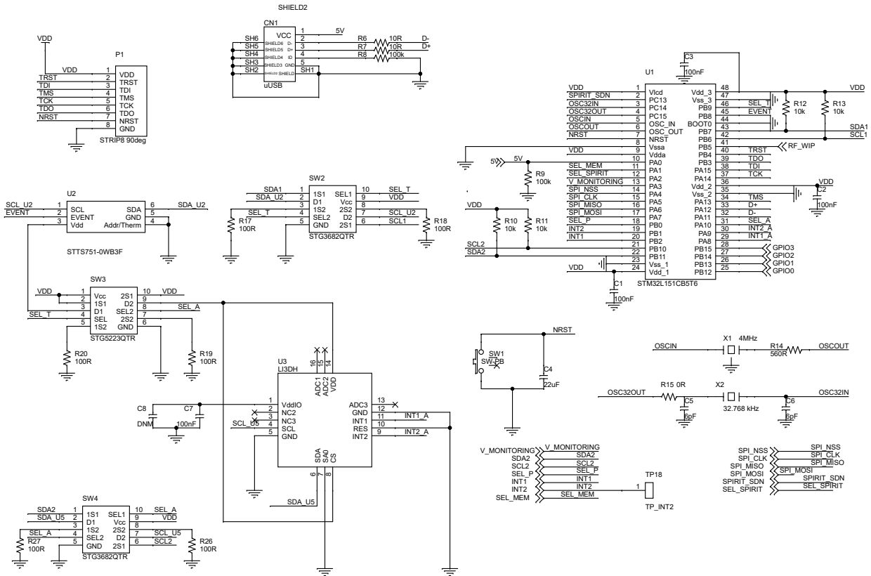
Figure 4: STDES-ERH003V1 transmitter board schematic (4 of 4)
