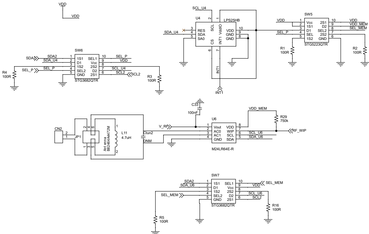
Figure 2: STDES-ERH003V1 transmitter board schematic (2 of 4)
