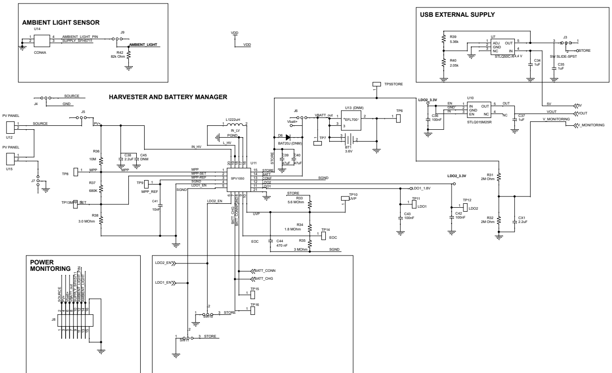
Figure 4: STDES-ERH003V1 transmitter board schematic (4 of 4)
