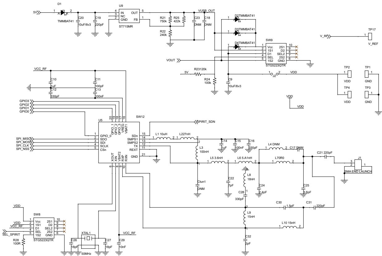
Figure 2: STDES-ERH003V1 transmitter board schematic (2 of 4)
