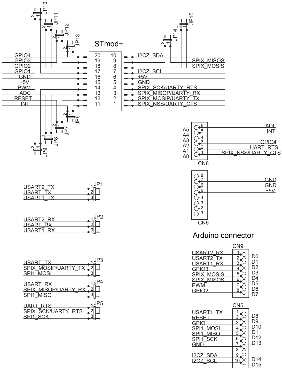
Figure 1: X-NUCLEO-STMODA1 circuit schematics
