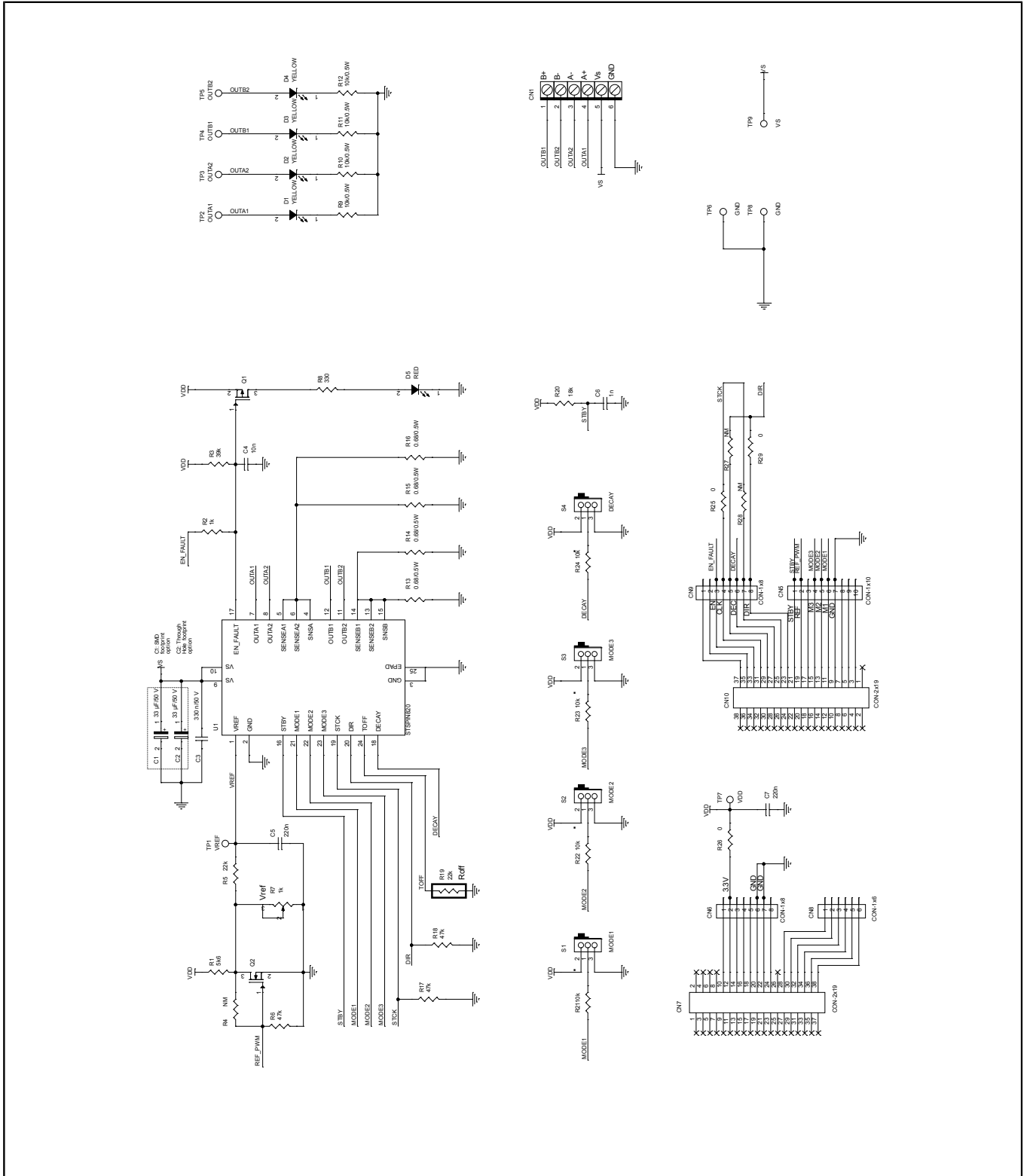
Figure 1: X-NUCLEO-IHM14A1 circuit schematic
