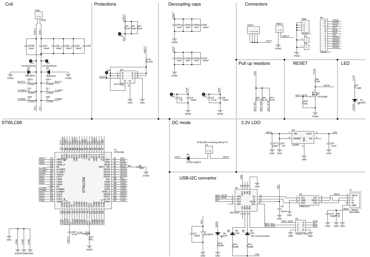
Figure 1: STEVAL-ISB68RX schematic diagrams
