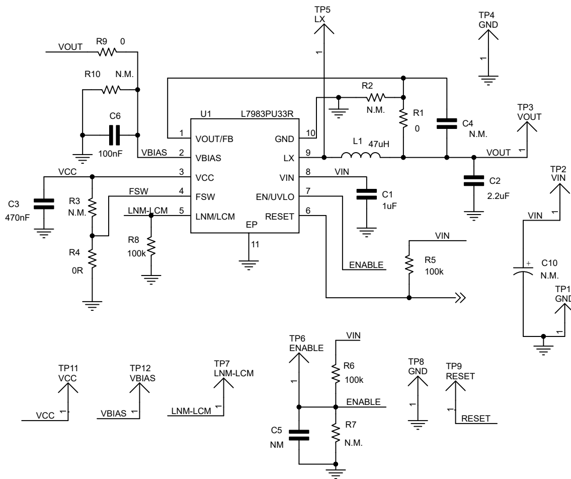
Figure 1: STEVAL-L7983V33 board schematic
