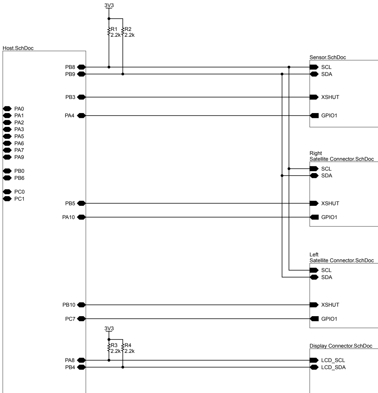
Figure 1. X-NUCLEO-53L4A2 circuit schematic (1 of 6)
