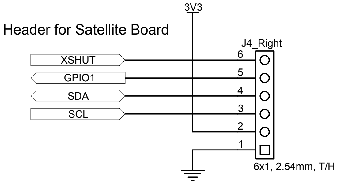
Figure 6. X-NUCLEO-53L4A2 circuit schematic (6 of 6)
