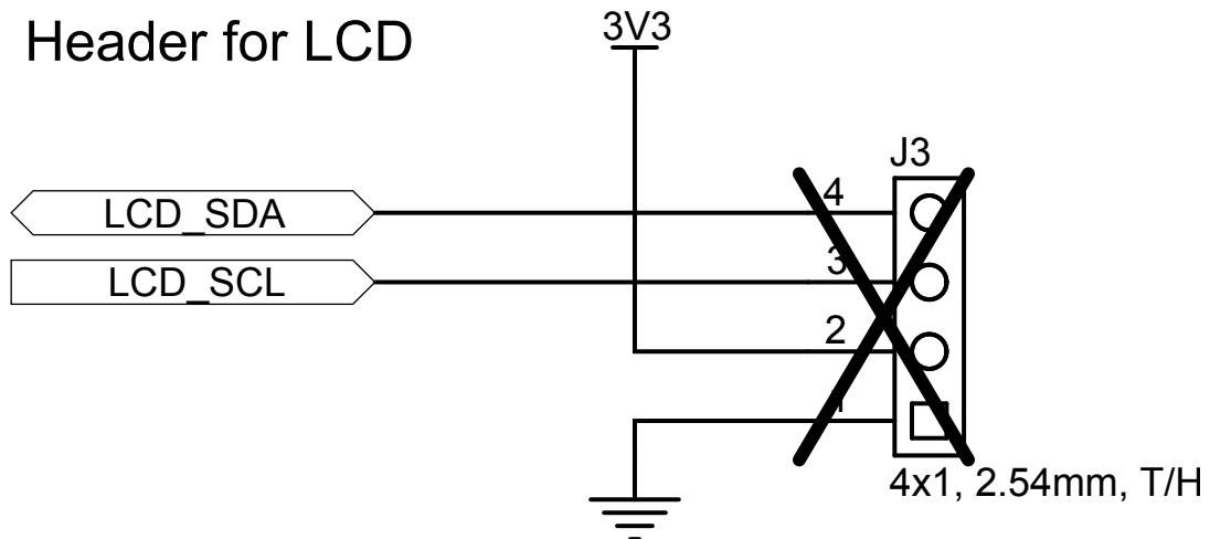
Figure 4. X-NUCLEO-53L4A2 circuit schematic (4 of 6)
