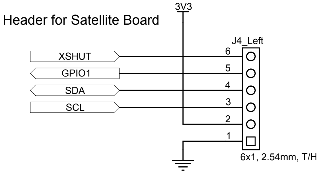
Figure 5. X-NUCLEO-53L4A2 circuit schematic (5 of 6)
