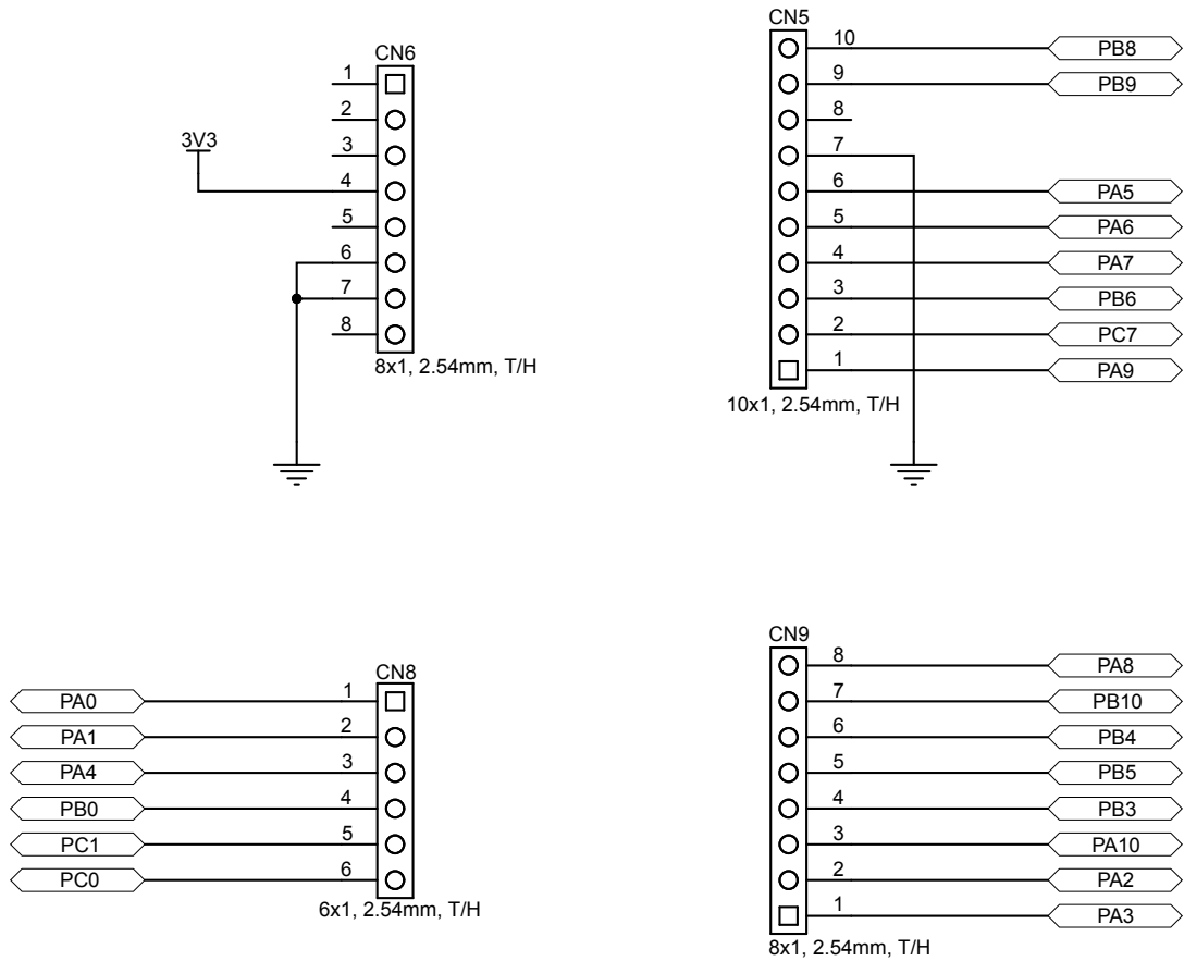
Figure 4. X-NUCLEO-53L4A2 circuit schematic (4 of 6)
