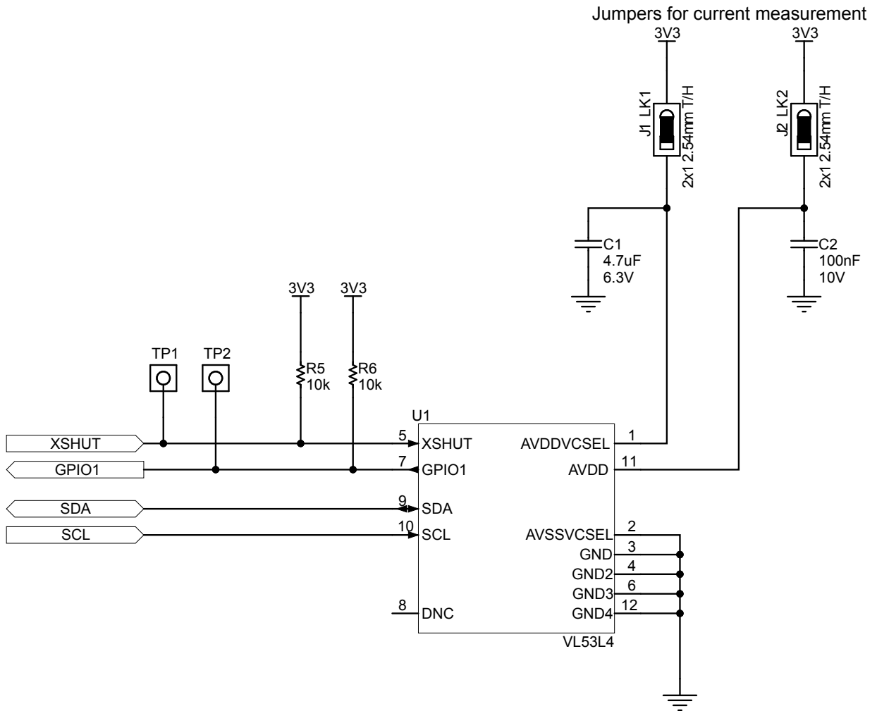
Figure 2. X-NUCLEO-53L4A2 circuit schematic (2 of 6)
