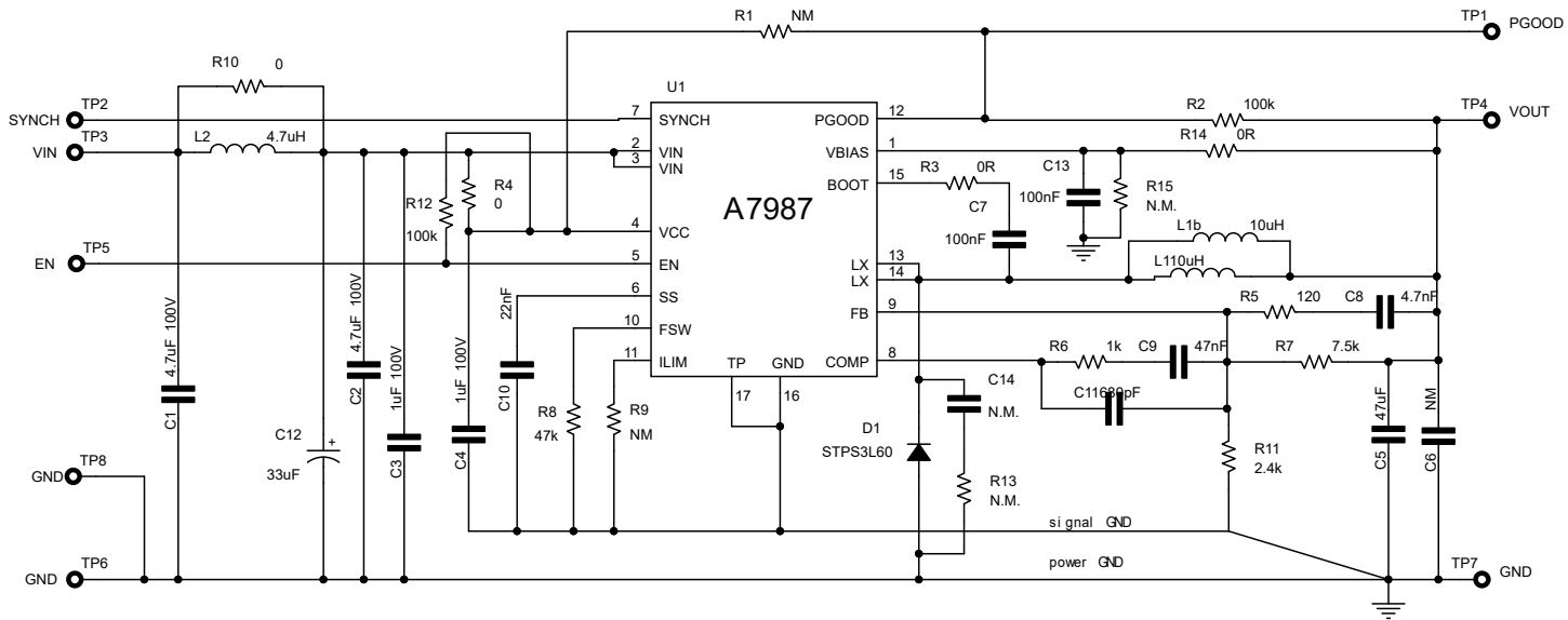
Figure 1: STEVAL-ISA207V1 board schematic
