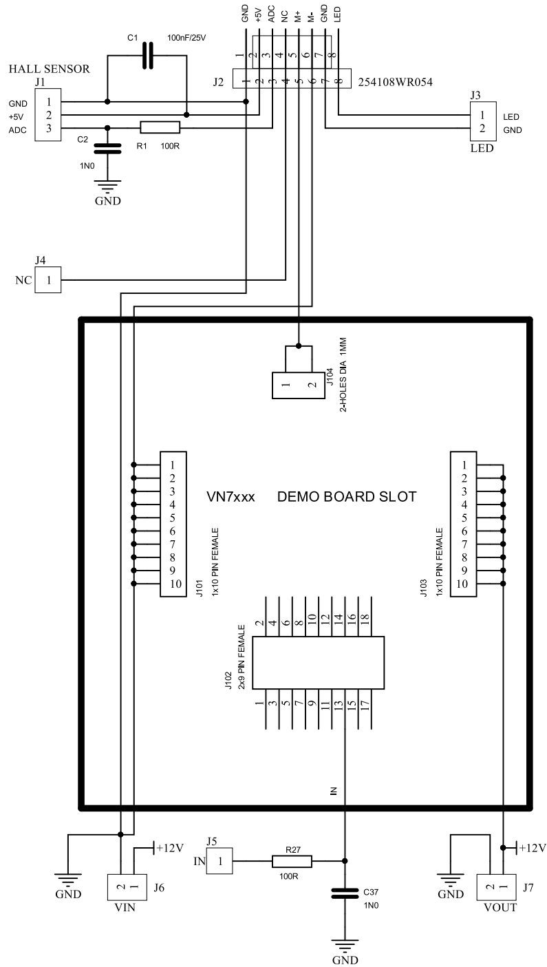
Figure 1: AEK-CON-BSPOTV1 schematic
