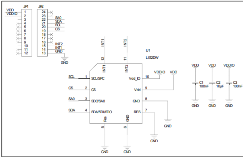
Figure 1: STEVAL-MKI179V1 circuit schematic
