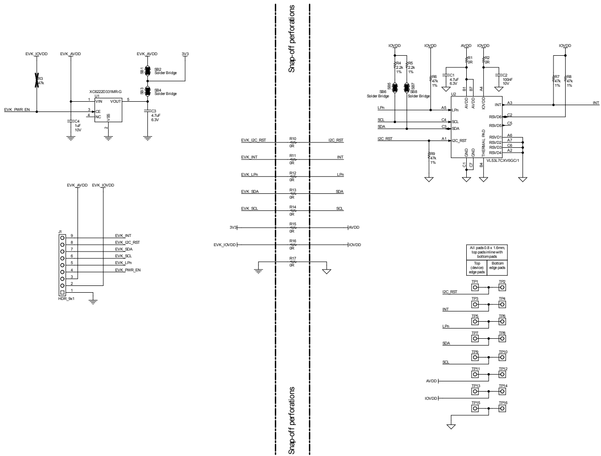
Figure 1. SATEL-VL53L7CX circuit schematic
