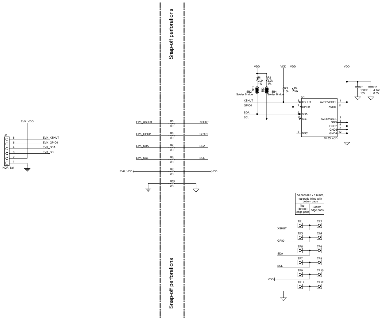
Figure 1. SATEL-VL53L4CD circuit schematic
