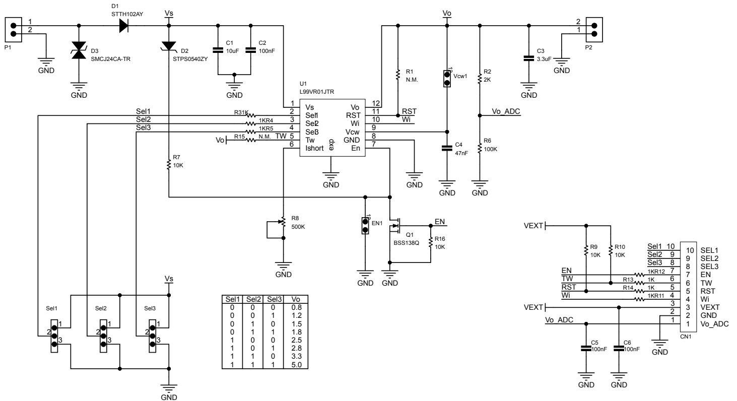
Figure 1. AEK-POW-LDOV01J circuit schematic
