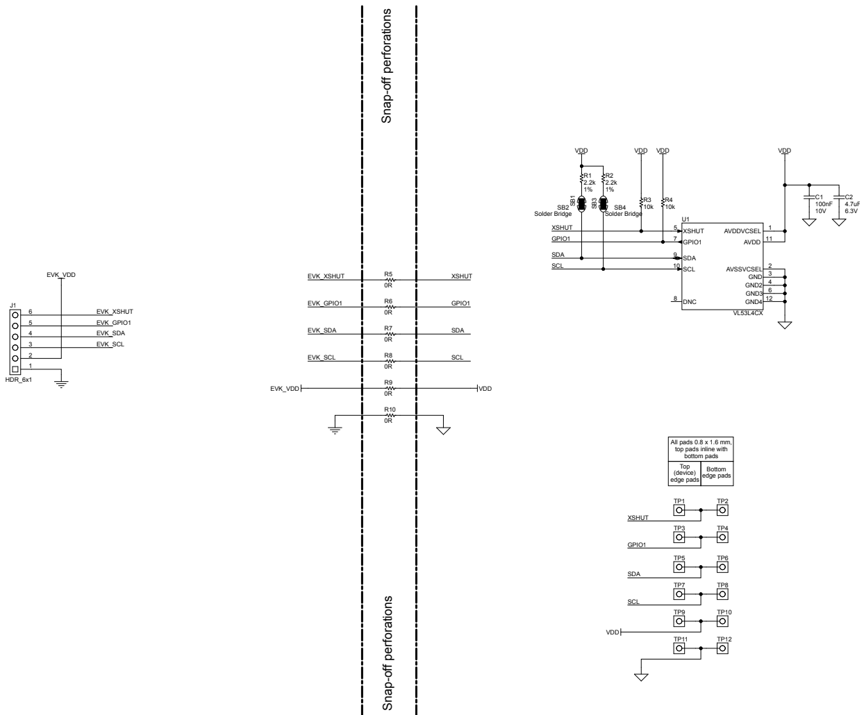
Figure 1. SATEL-VL53L4CX circuit schematic
