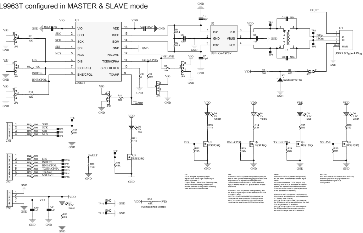
Figure 1. AEK-COM-ISOSPI1 circuit schematic
