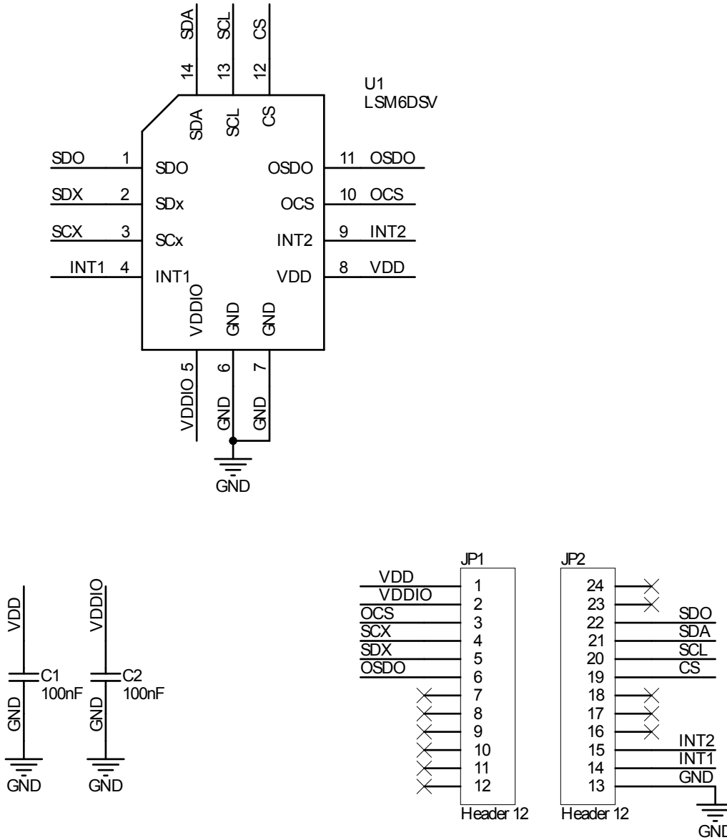
Figure 1. STEVAL-MKI239A circuit schematic
