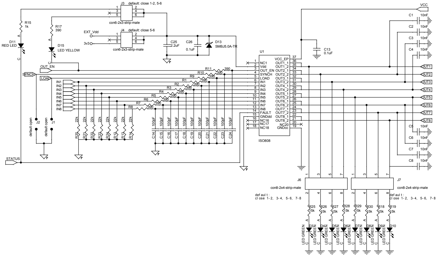
Figure 2. X-NUCLEO-OUT11A1 circuit schematic (2 of 2)
