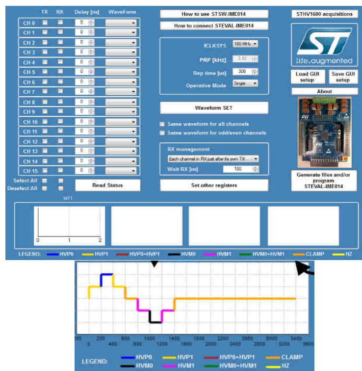
GUI – HV waveforms builder
