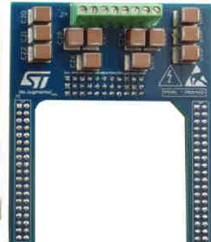
3. STEVAL-IME014V1D
